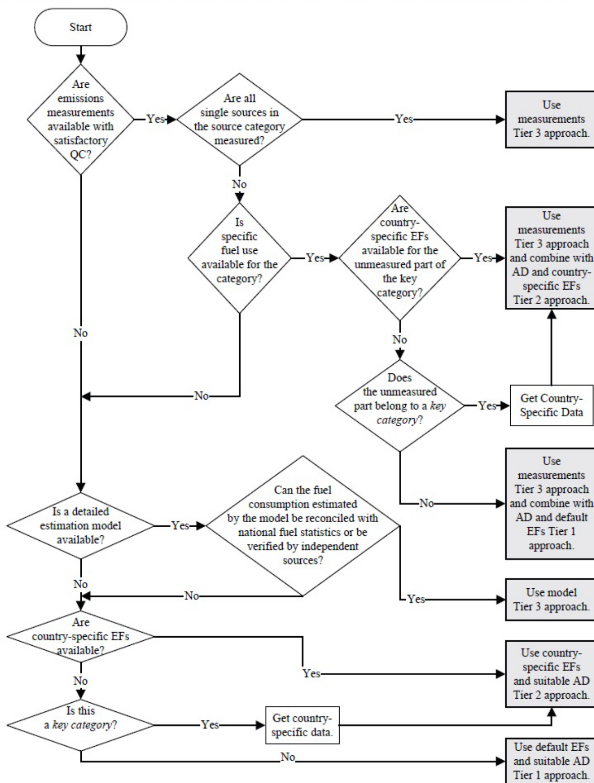
Figure 1.2 Generalised decision tree for estimating emissions from fuel combustion
